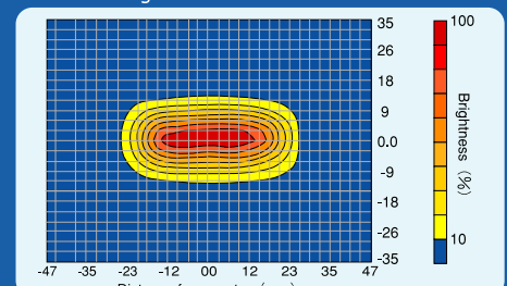
UB-50R15 Light distribution at WD 10mm
