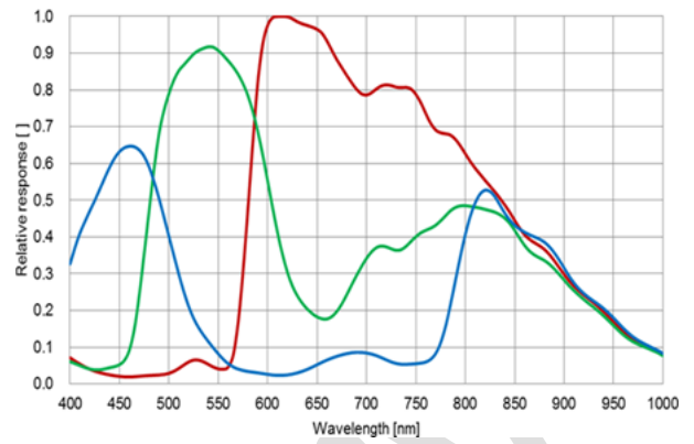
Pregius's IMX250 Color Spectral Response
